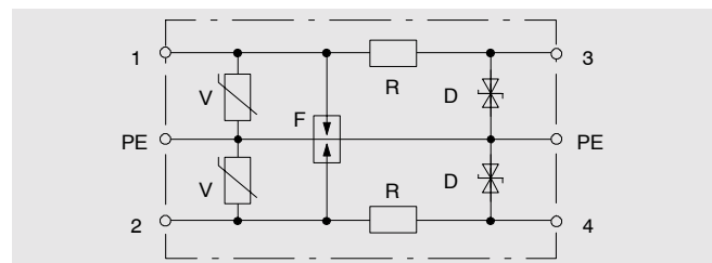
Block diagram of FRD 2
