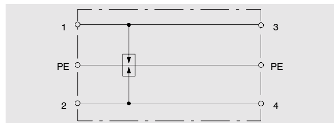
Block diagram of TKS-B
