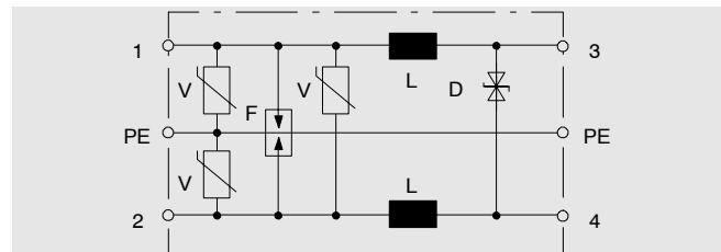
Block diagram of FLD
